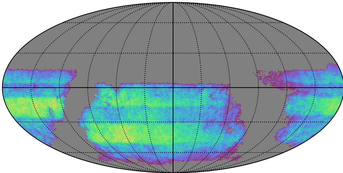
baseline_v2.1_10yrs i band non-DD year 5: ExgalM5WithCuts
