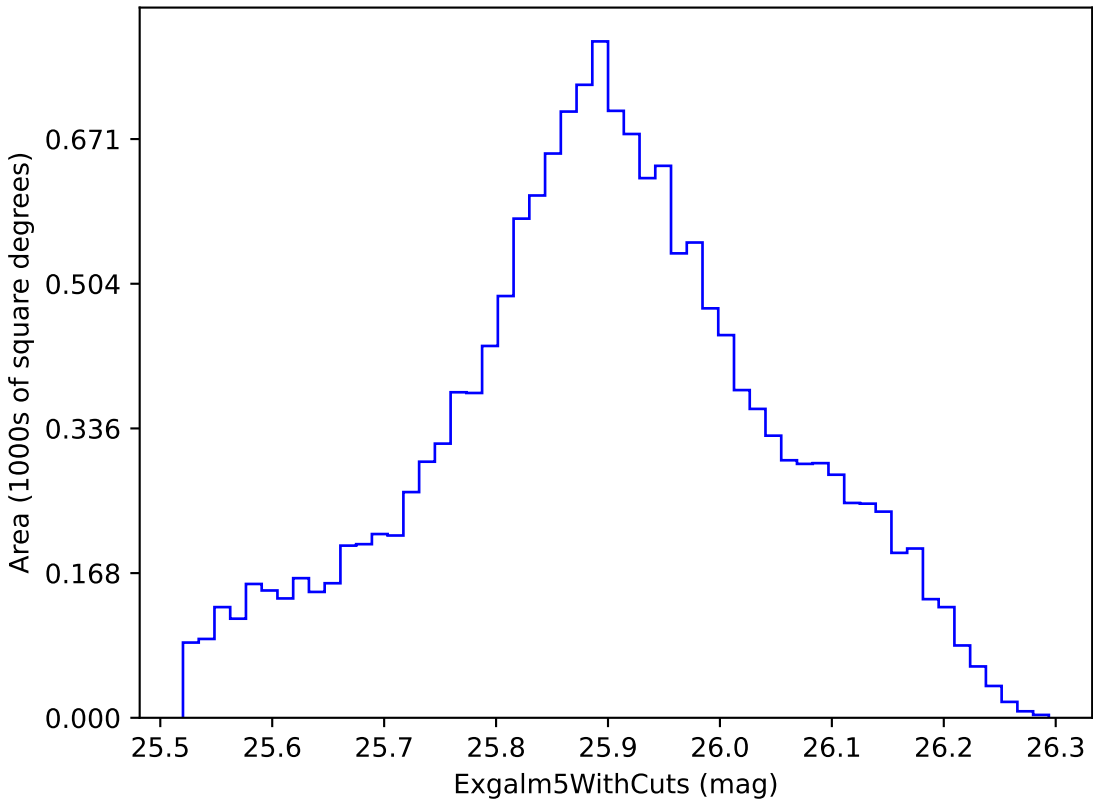
baseline_v2.1_10yrs i band non-DD year 5: ExgalM5WithCuts
