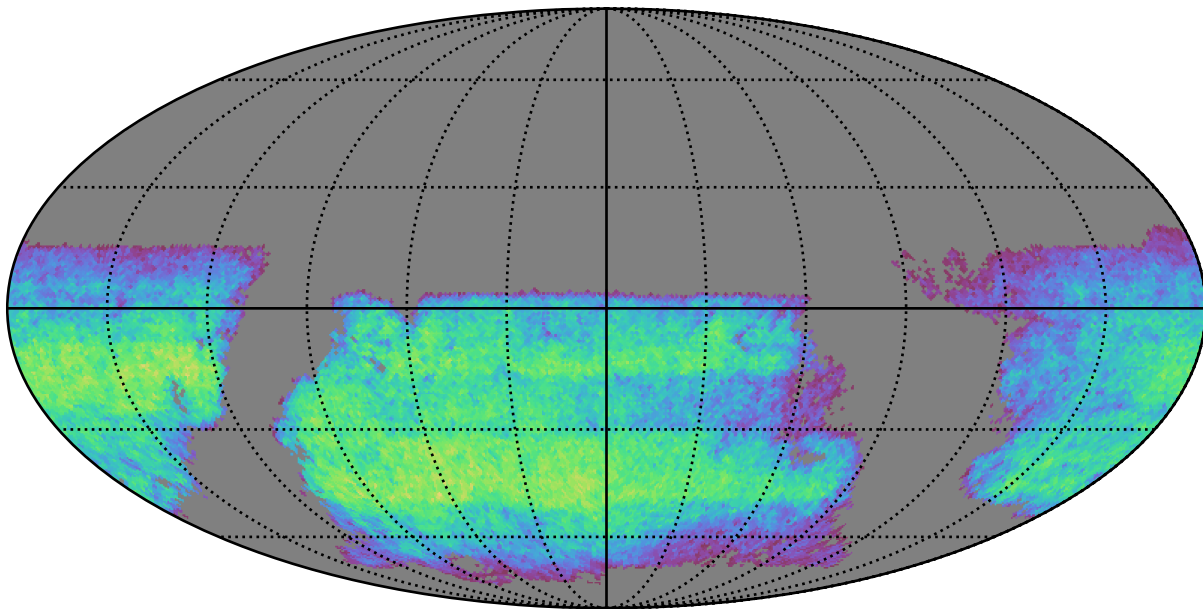
baseline_v2.1_10yrs i band non-DD year 4: ExgalM5WithCuts
