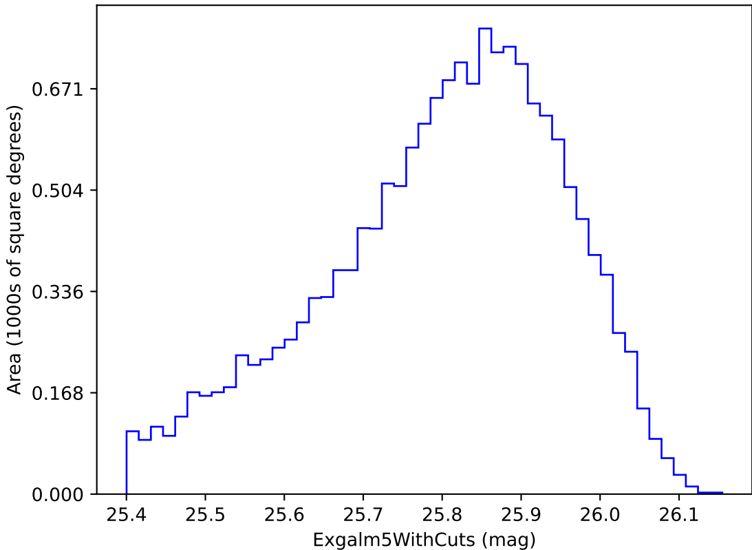
baseline_v2.1_10yrs i band non-DD year 4: ExgalM5WithCuts
