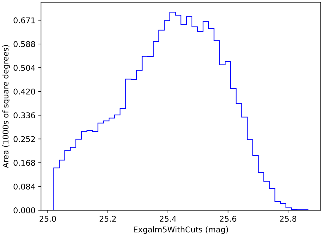
baseline_v2.1_10yrs i band non-DD year 2: ExgalM5WithCuts
