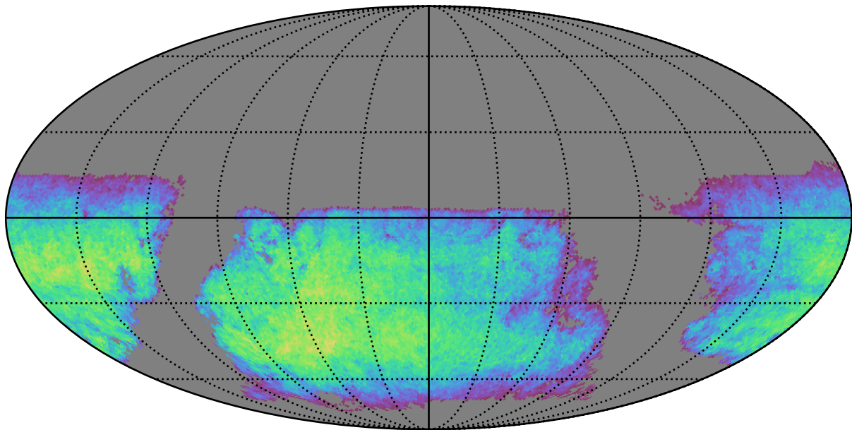
baseline_v2.1_10yrs i band non-DD year 10: ExgalM5WithCuts
