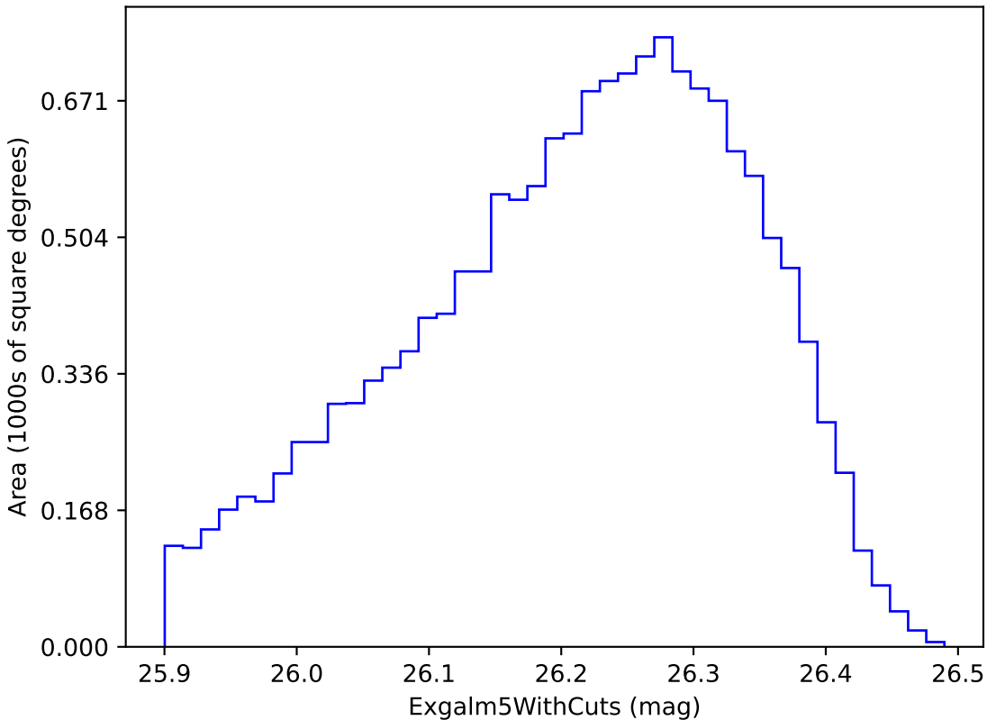
baseline_v2.1_10yrs i band non-DD year 10: ExgalM5WithCuts
