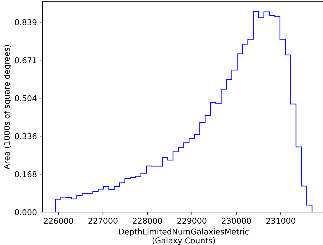
baseline_v2.1_10yrs i band galaxies non-DD: DepthLimitedNumGalaxiesMetric
