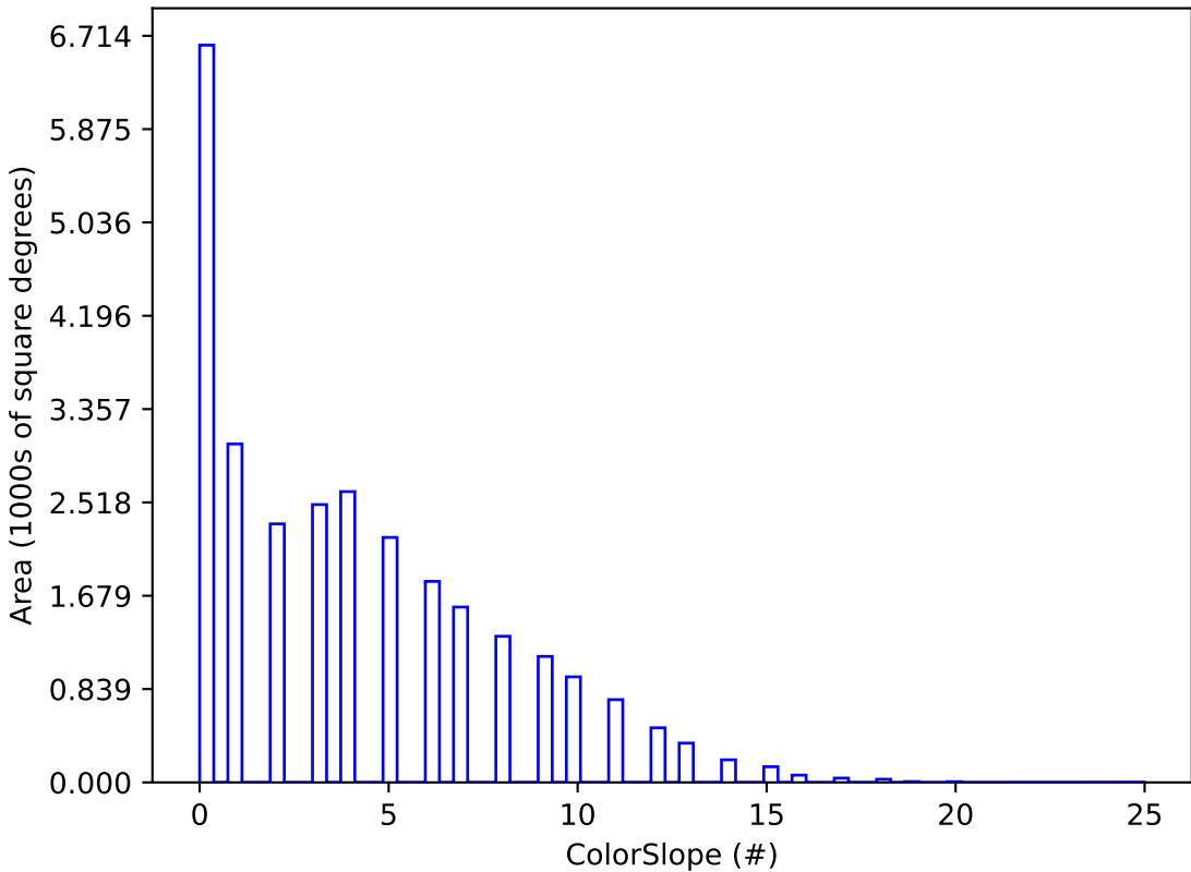
baseline_v2.1_10yrs visitExposureTime > 19: ColorSlope
