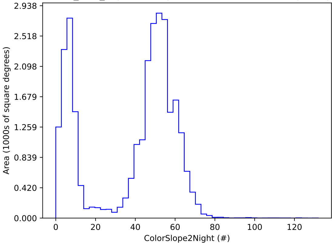
baseline_v2.1_10yrs visitExposureTime > 19: ColorSlope2Night
