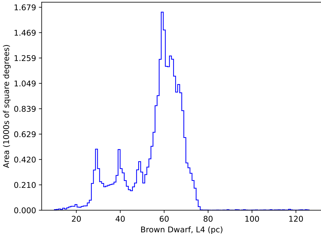
baseline_v2.1_10yrs : Brown Dwarf, L4
