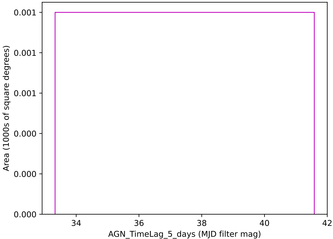
baseline_v2.1_10yrs z band: AGN_TimeLag_5_days
