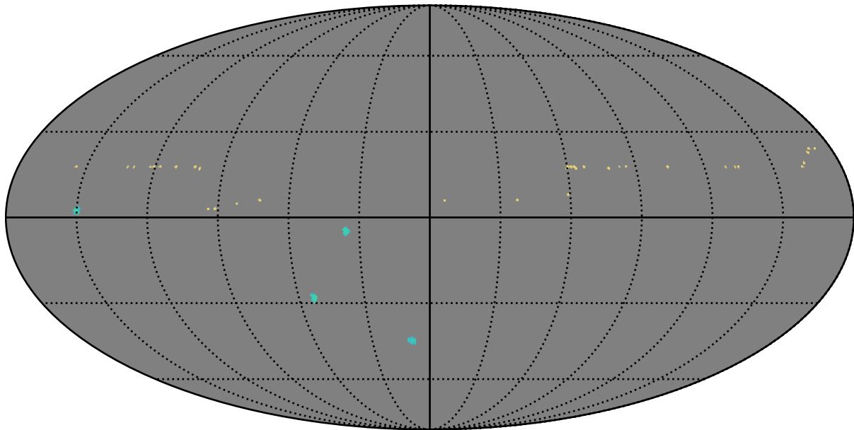
baseline_v2.1_10yrs y band: AGN_TimeLag_5_days
