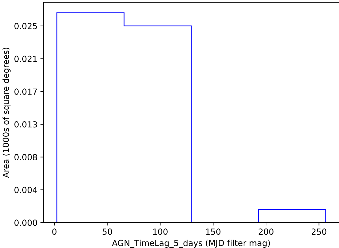
baseline_v2.1_10yrs y band: AGN_TimeLag_5_days
