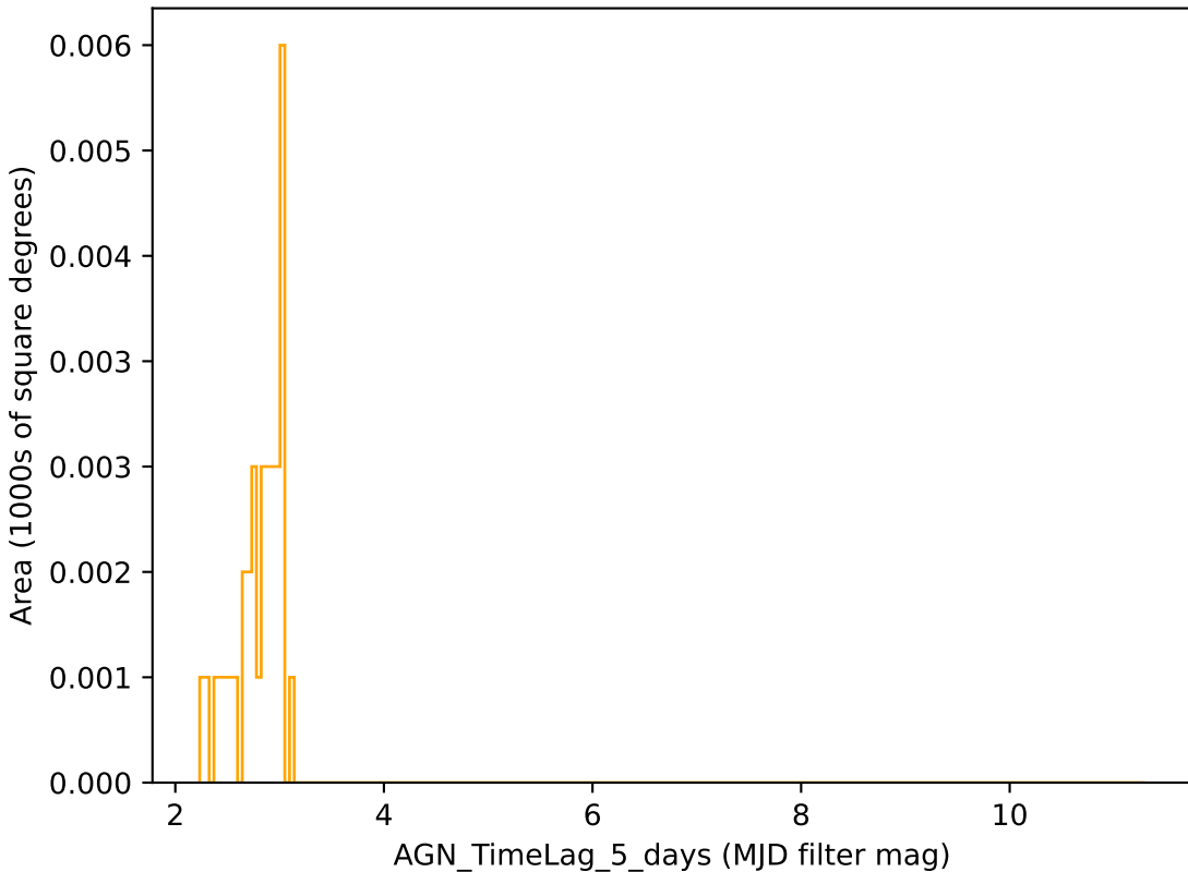
baseline_v2.1_10yrs r band: AGN_TimeLag_5_days
