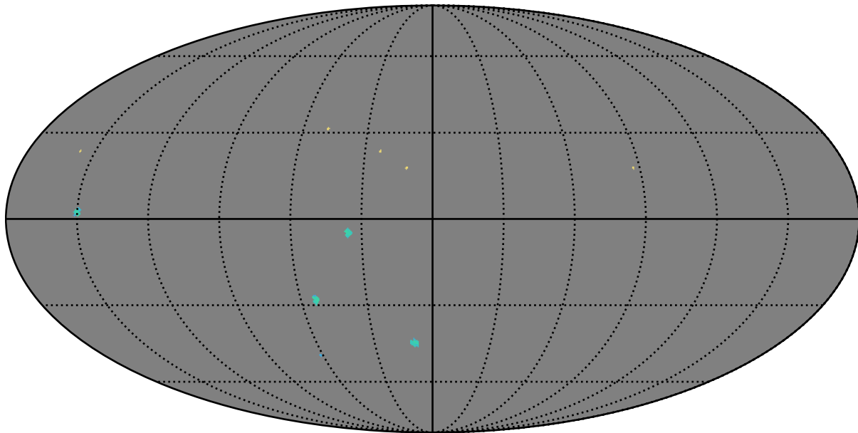
baseline_v2.1_10yrs i band: AGN_TimeLag_5_days
