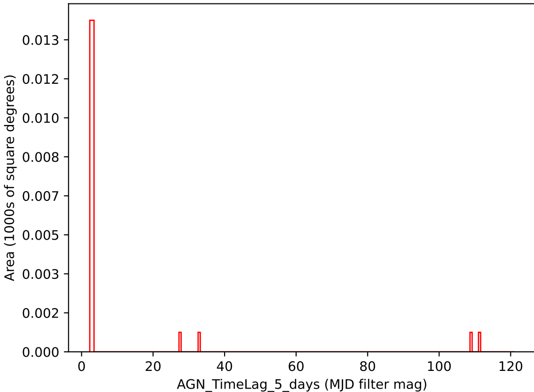
baseline_v2.1_10yrs i band: AGN_TimeLag_5_days
