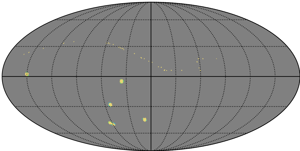
baseline_v2.1_10yrs all bands: AGN_TimeLag_5_days
