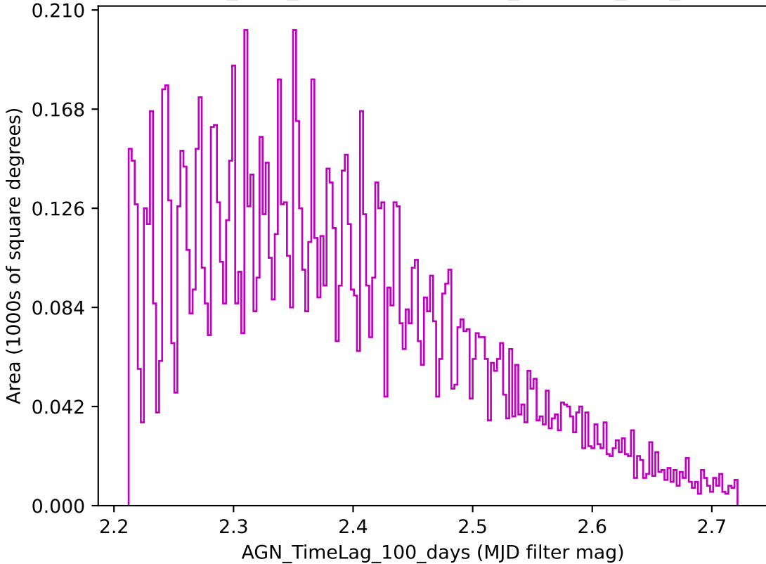
baseline_v2.1_10yrs z band: AGN_TimeLag_100_days
