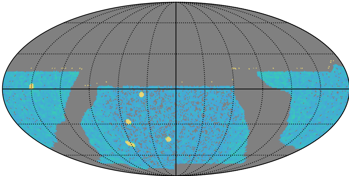
baseline_v2.1_10yrs y band: AGN_TimeLag_100_days
