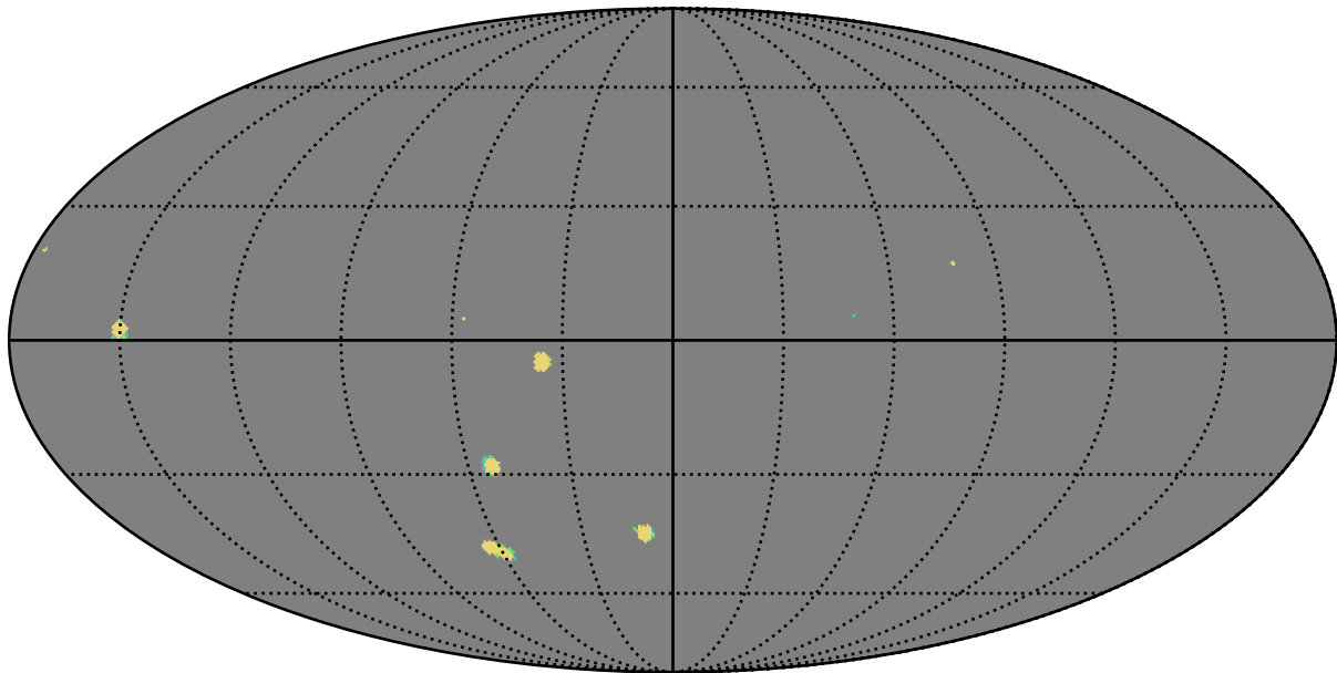
baseline_v2.1_10yrs u band: AGN_TimeLag_100_days
