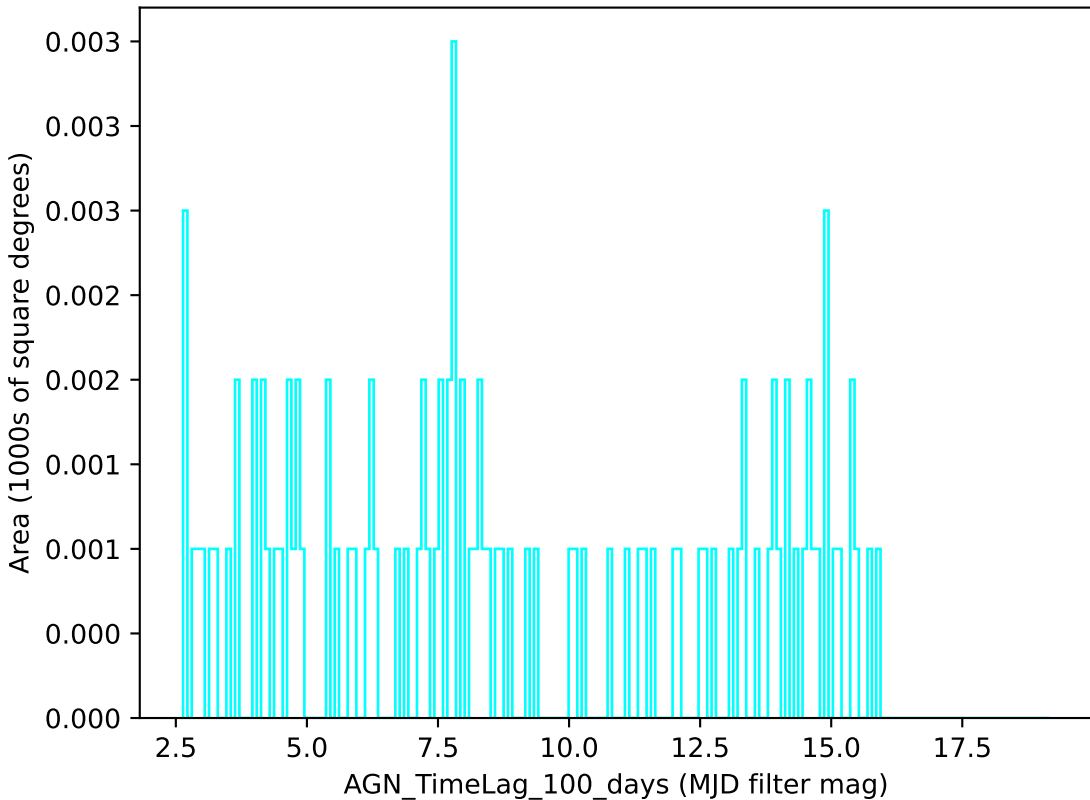
baseline_v2.1_10yrs u band: AGN_TimeLag_100_days
