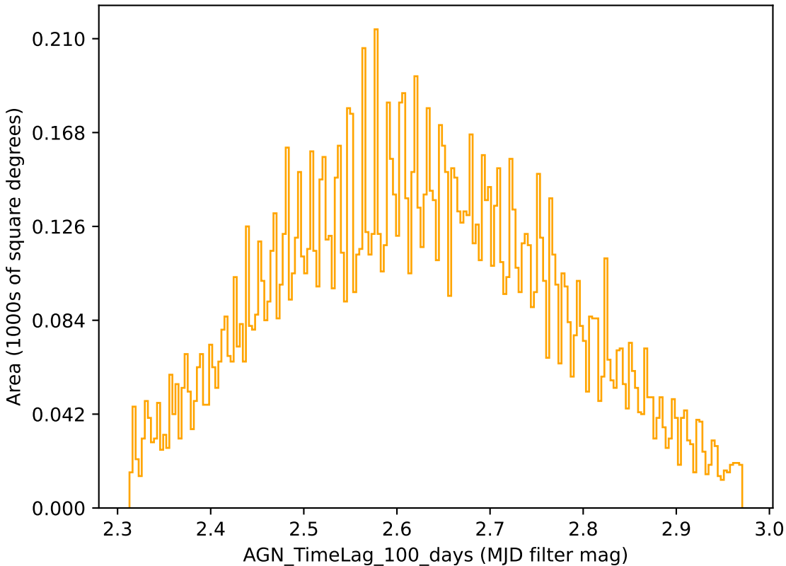
baseline_v2.1_10yrs r band: AGN_TimeLag_100_days
