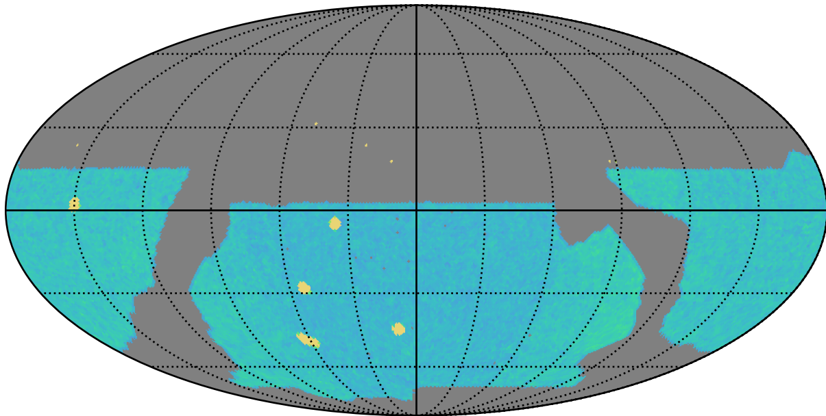
baseline_v2.1_10yrs i band: AGN_TimeLag_100_days
