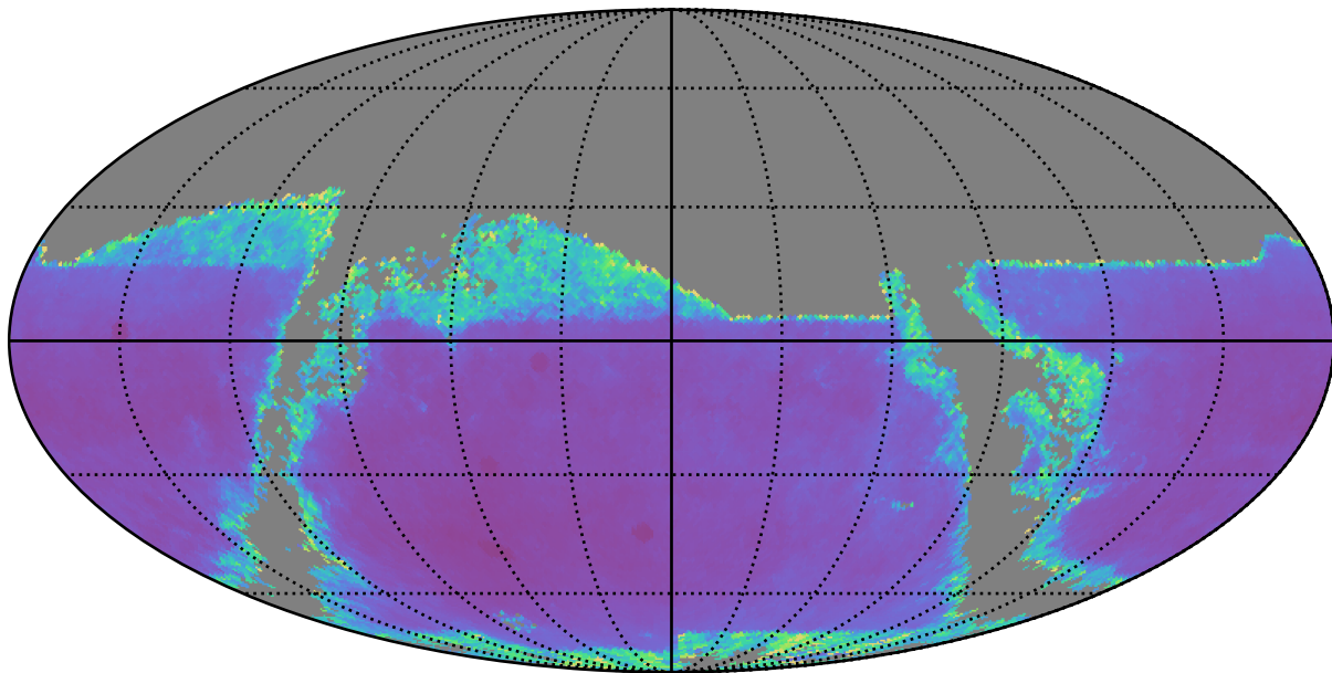
baseline_v2.1_10yrs z band: AGN SF_uncert
