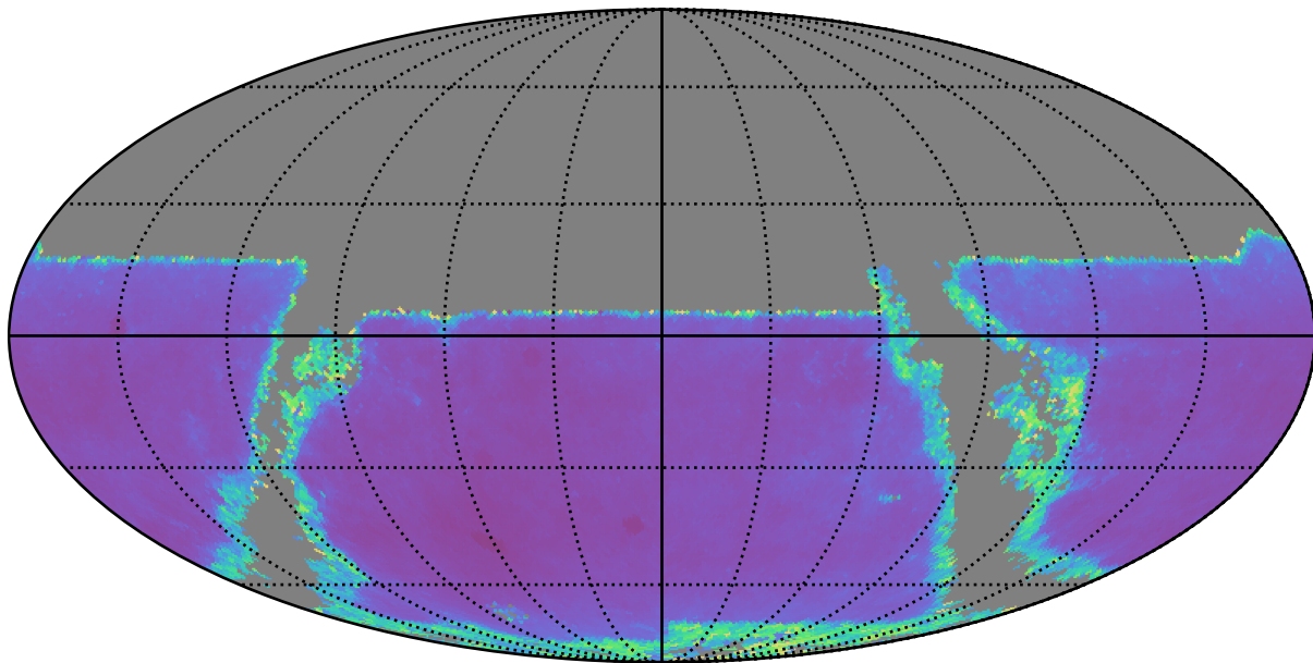
baseline_v2.1_10yrs y band: AGN SF_uncert
