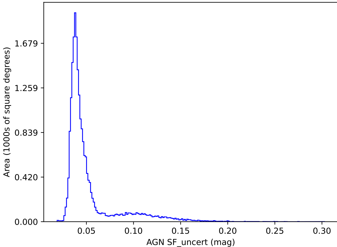
baseline_v2.1_10yrs y band: AGN SF_uncert
