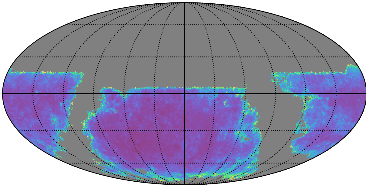
baseline_v2.1_10yrs u band: AGN SF_uncert
