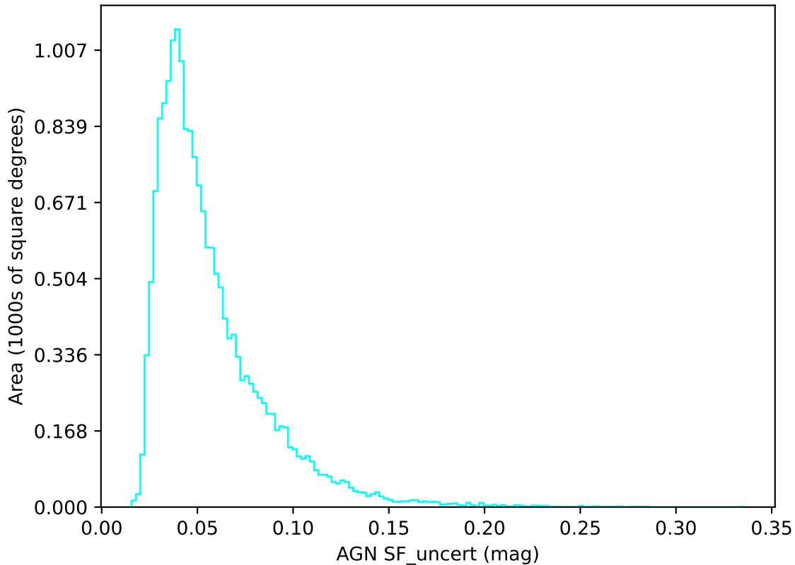
baseline_v2.1_10yrs u band: AGN SF_uncert
