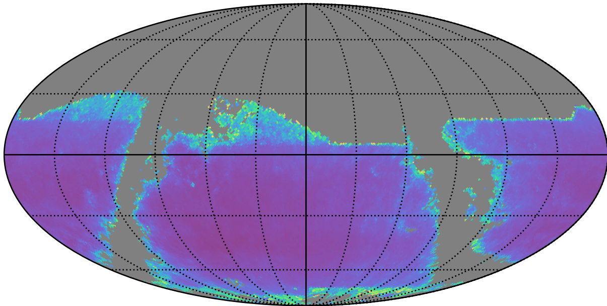
baseline_v2.1_10yrs r band: AGN SF_uncert
