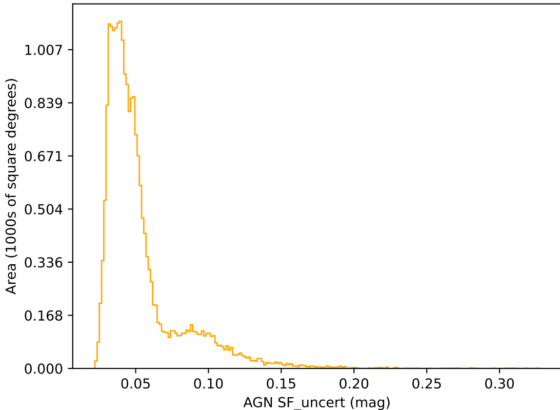
baseline_v2.1_10yrs r band: AGN SF_uncert
