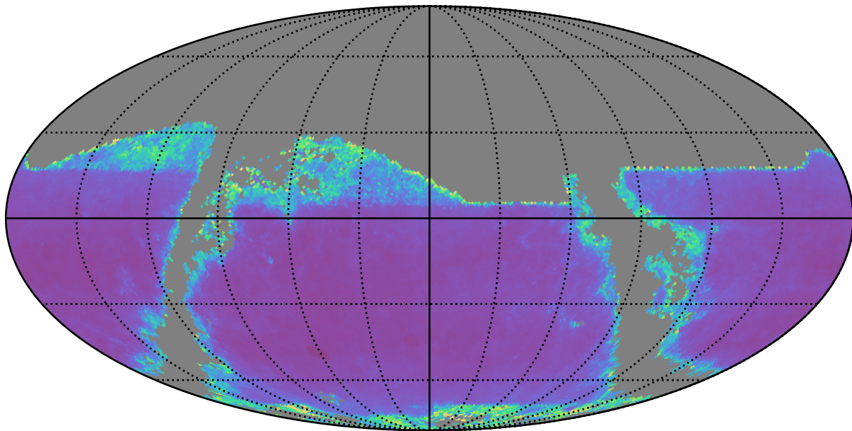
baseline_v2.1_10yrs i band: AGN SF_uncert
