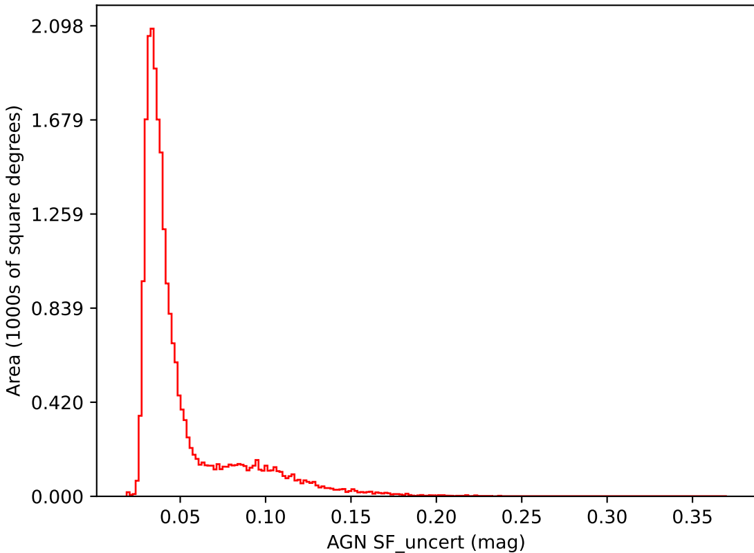
baseline_v2.1_10yrs i band: AGN SF_uncert
