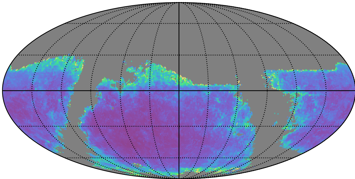
baseline_v2.1_10yrs g band: AGN SF_uncert
