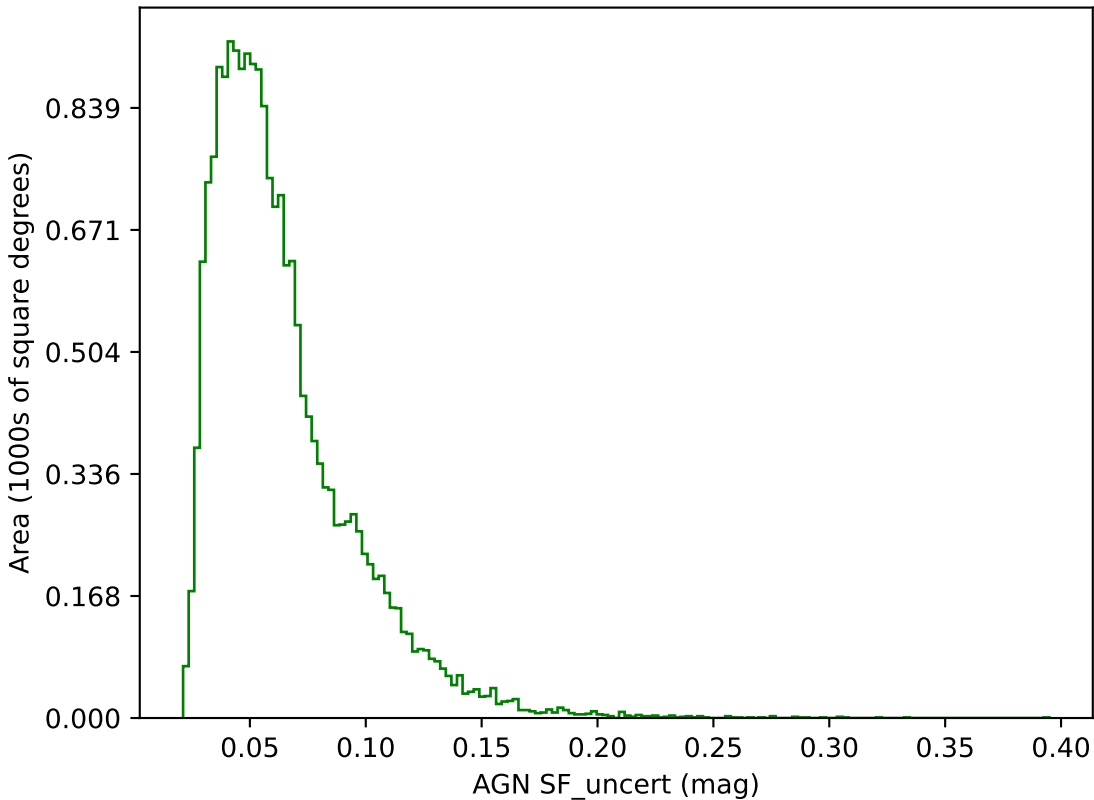
baseline_v2.1_10yrs g band: AGN SF_uncert
