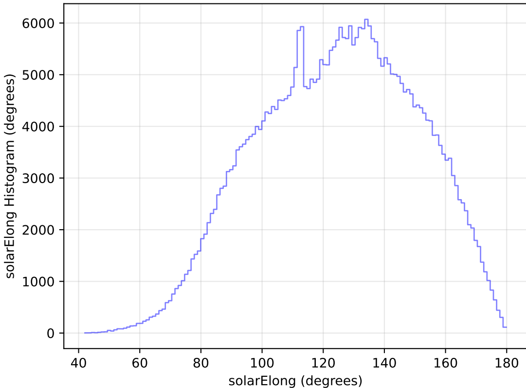
baseline_v2.1_10yrs WFD y band: solarElong Histogram
