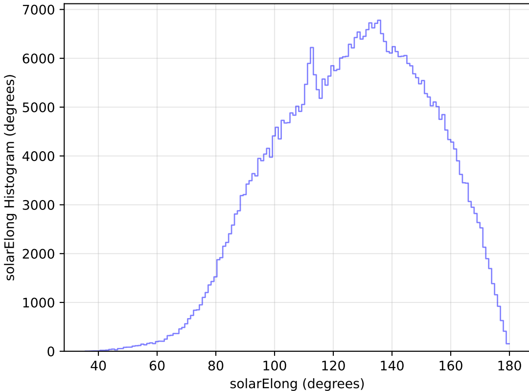
baseline_v2.1_10yrs WFD r band: solarElong Histogram
