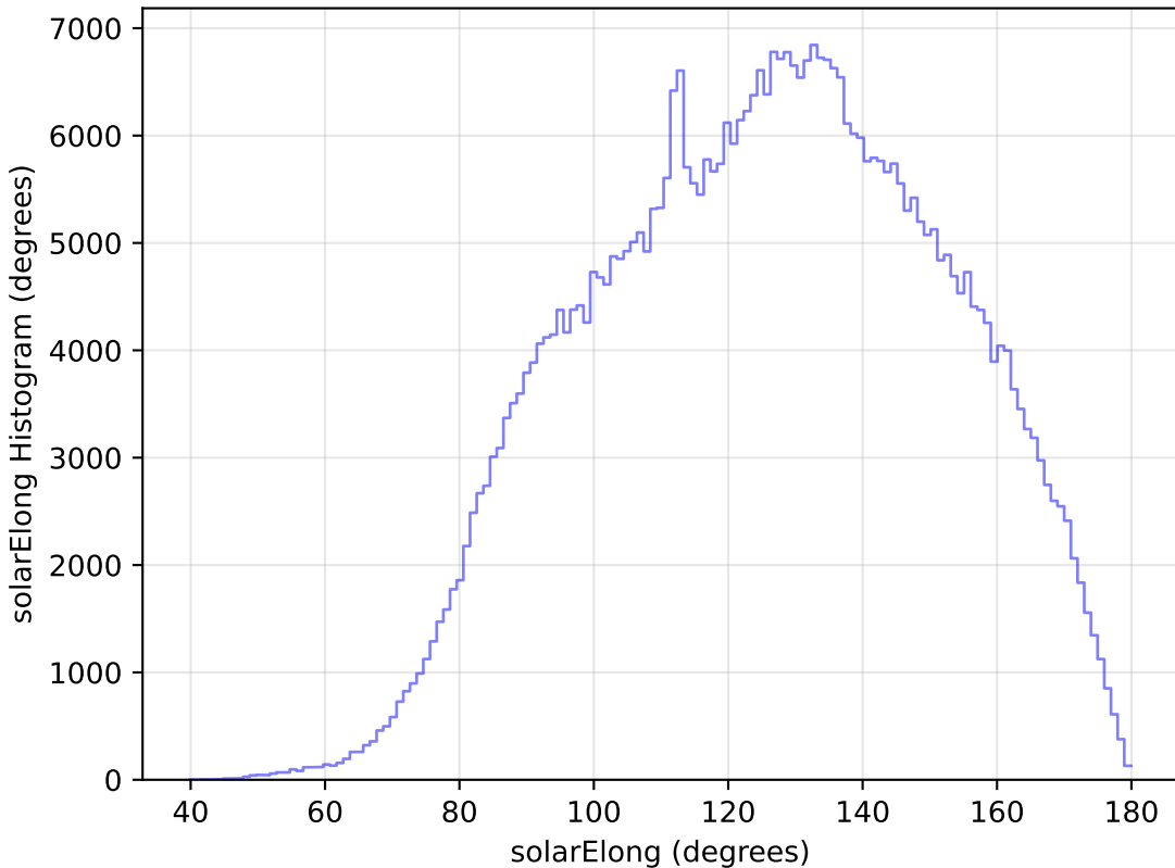
baseline_v2.1_10yrs WFD i band: solarElong Histogram
