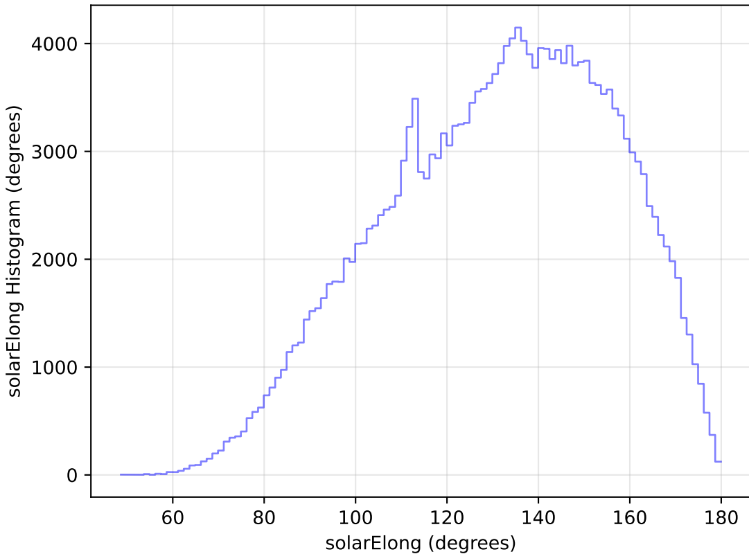
baseline_v2.1_10yrs WFD g band: solarElong Histogram
