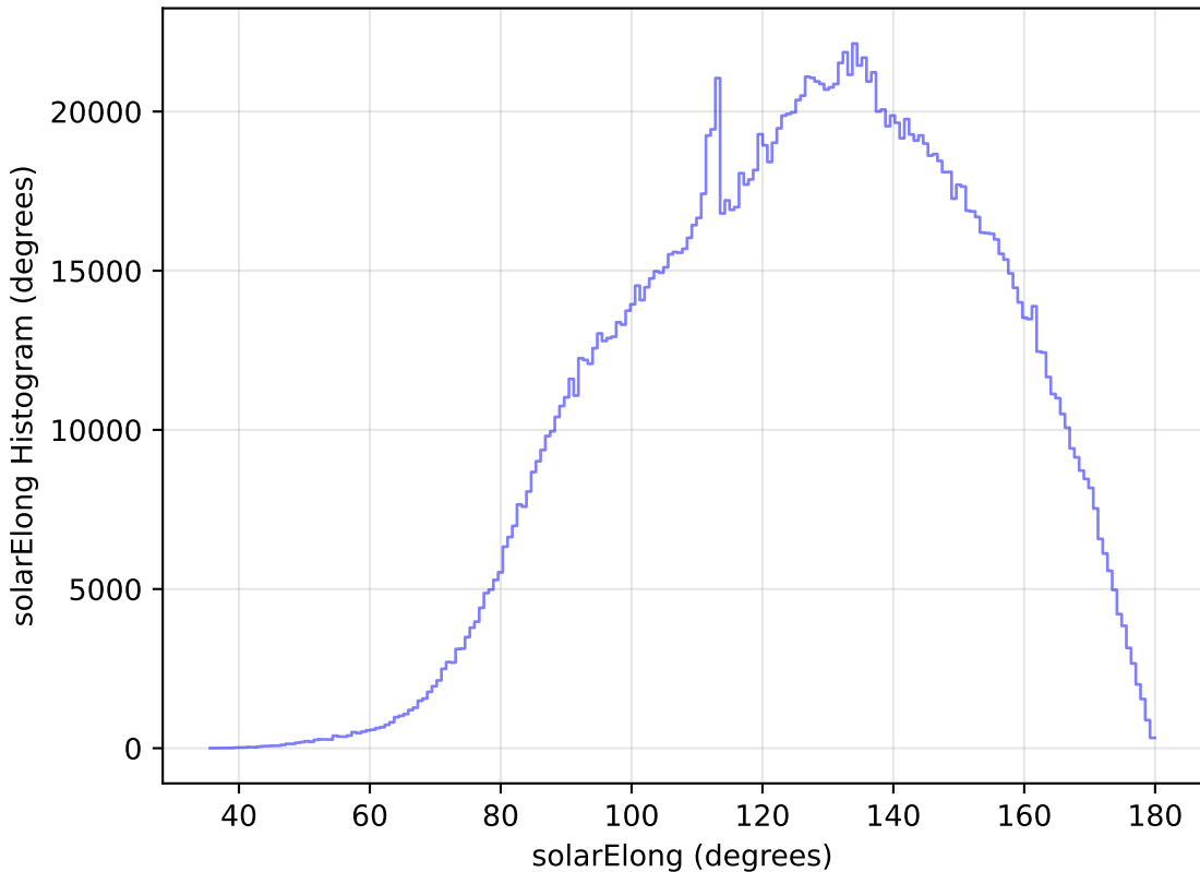
baseline_v2.1_10yrs WFD all bands: solarElong Histogram
