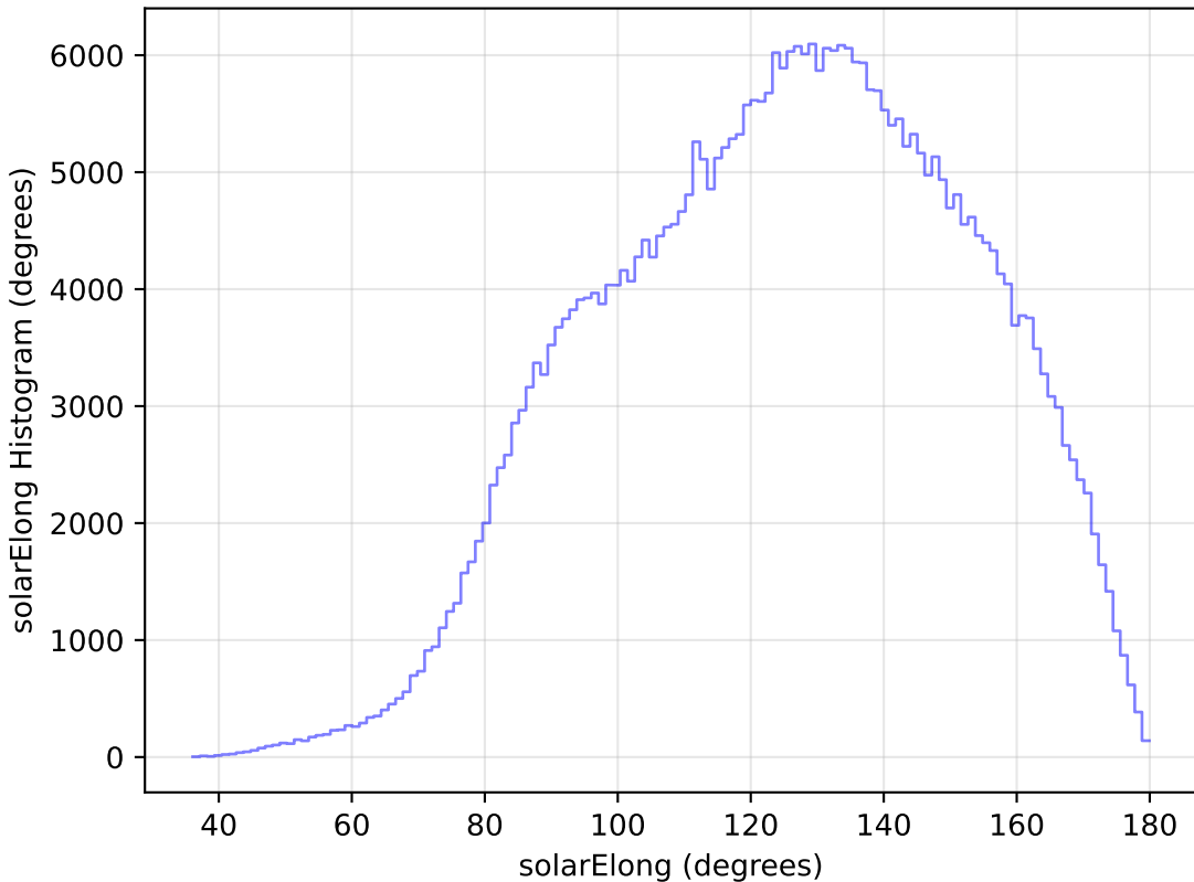
baseline_v2.1_10yrs All sky z band: solarElong Histogram
