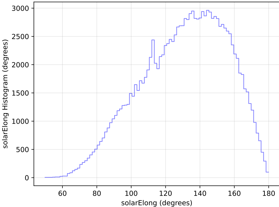
baseline_v2.1_10yrs All sky u band: solarElong Histogram
