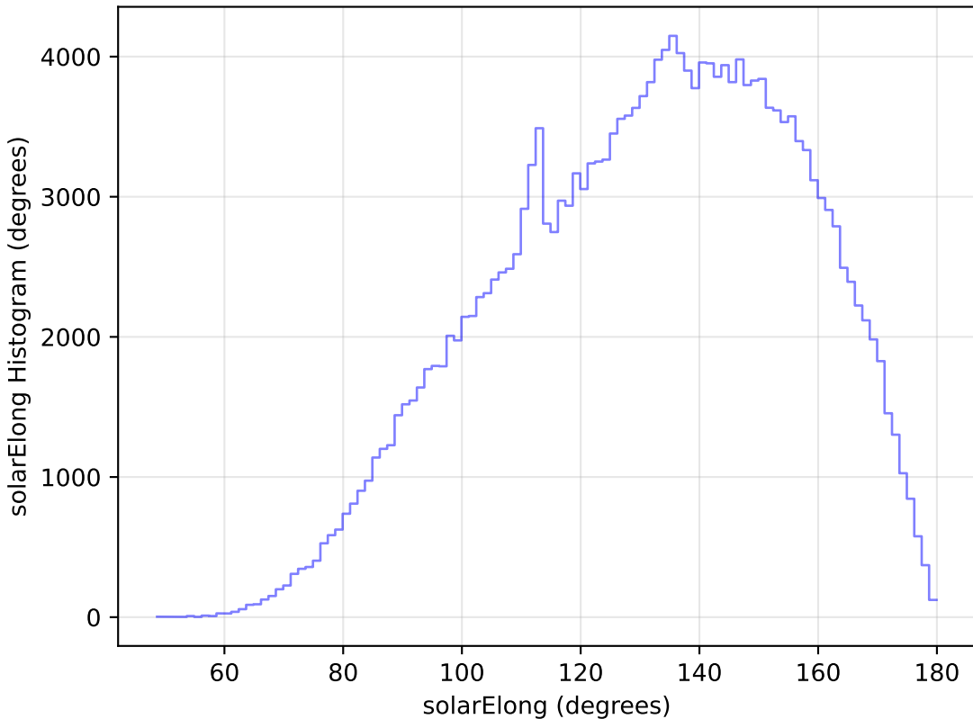
baseline_v2.1_10yrs All sky g band: solarElong Histogram
