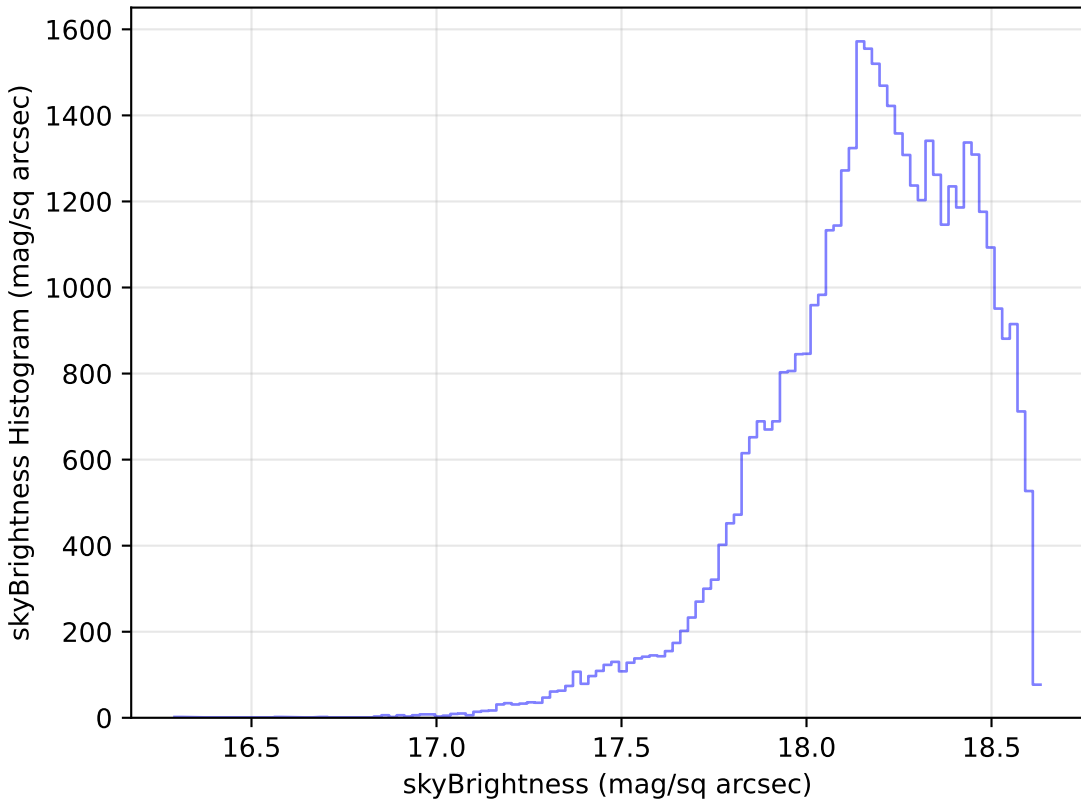
baseline_v2.1_10yrs Yr 1 y band: skyBrightness Histogram
