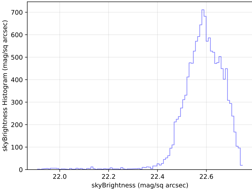
baseline_v2.1_10yrs Yr 1 u band: skyBrightness Histogram
