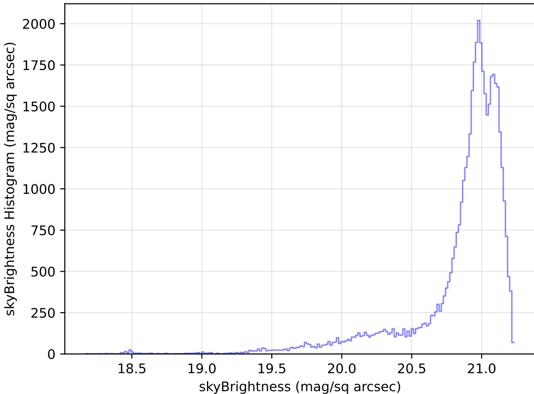
baseline_v2.1_10yrs Yr 1 r band: skyBrightness Histogram
