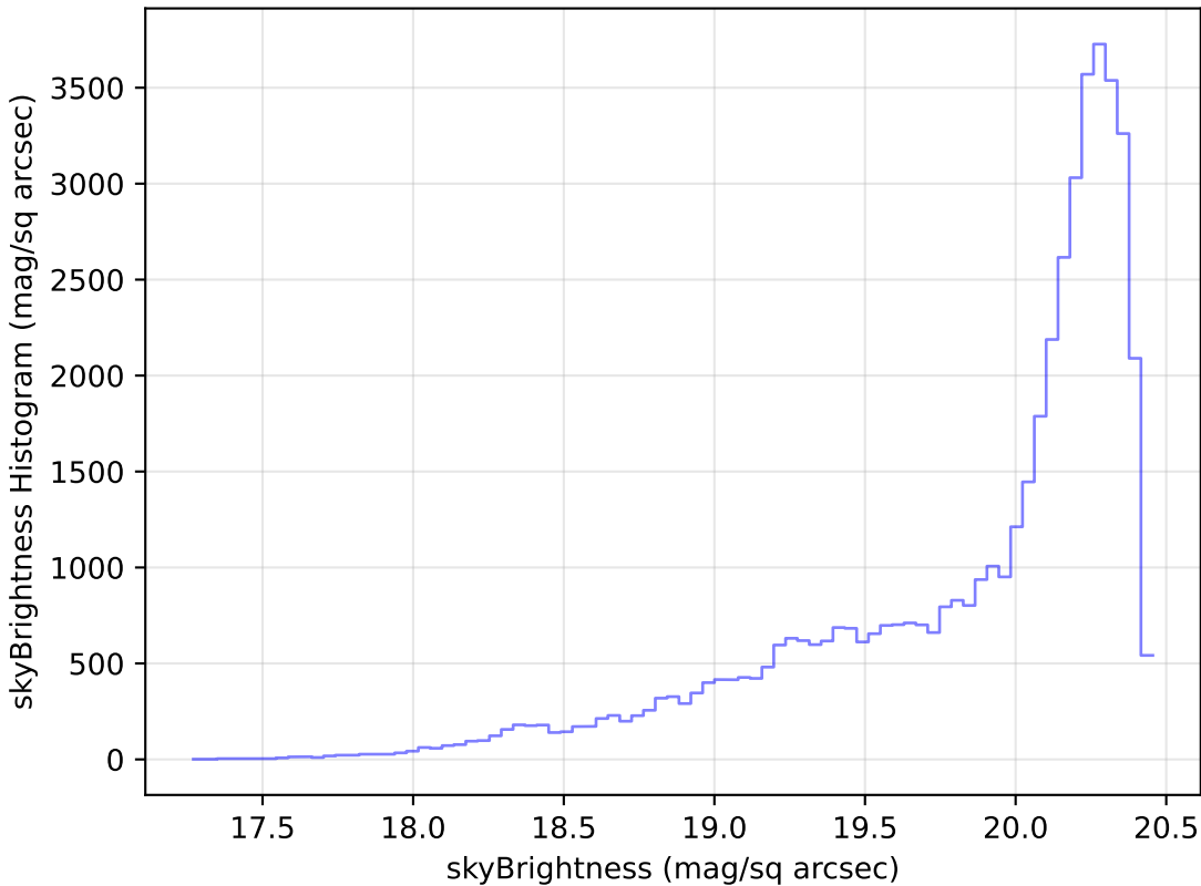
baseline_v2.1_10yrs Yr 1 i band: skyBrightness Histogram
