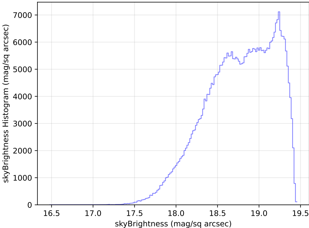
baseline_v2.1_10yrs WFD z band: skyBrightness Histogram
