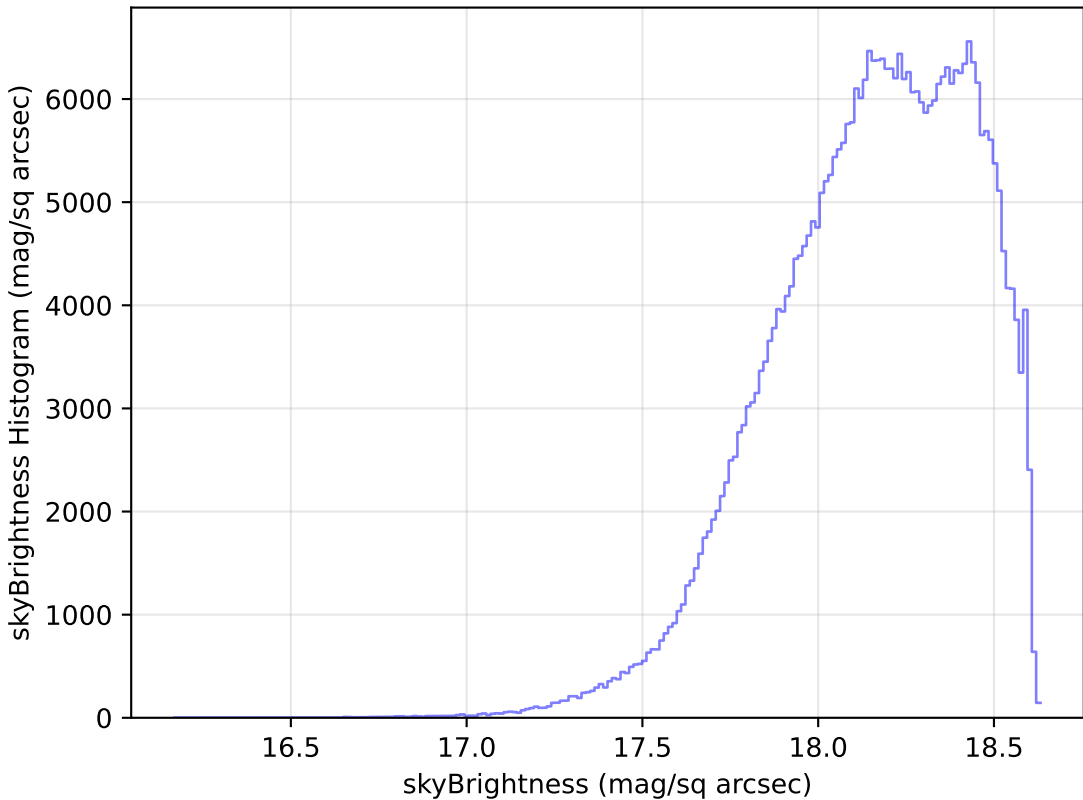
baseline_v2.1_10yrs WFD y band: skyBrightness Histogram
