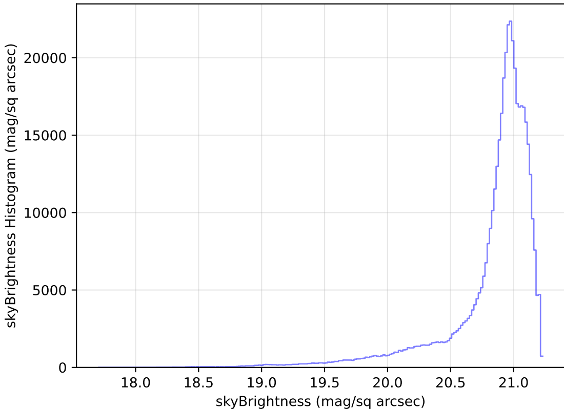
baseline_v2.1_10yrs WFD r band: skyBrightness Histogram
